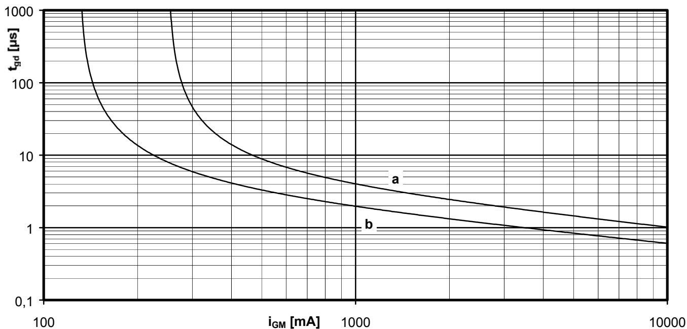
Zündverzugscharakteristik / Gate controlled delay time t_{gd} = f(i_G)
