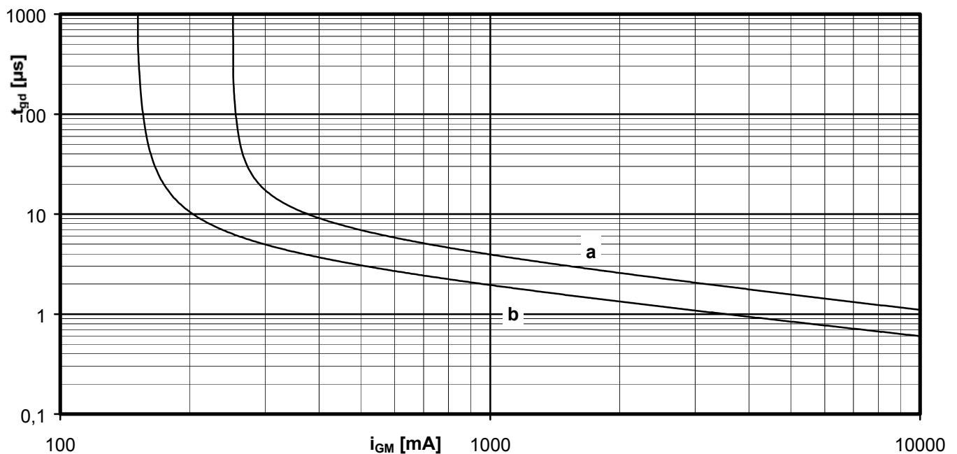
Zündverzugscharakteristik / Gate controlled delay time t_{gd} = f(i_G)
