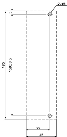
Mounting holes
