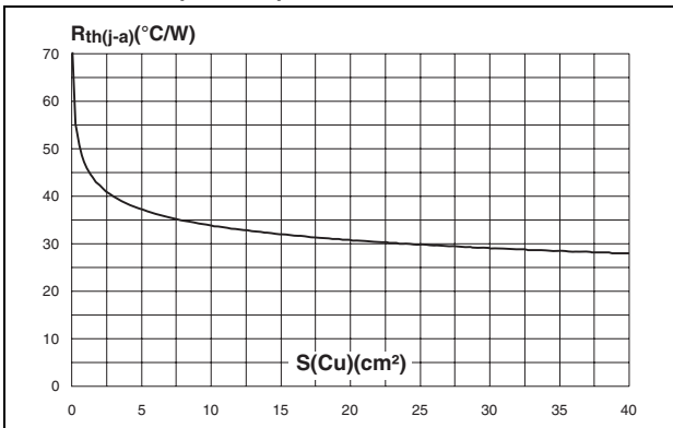
Figure 13. Thermal resistance junction to ambient versus copper surface under tab (epoxy FR4, e_{CU} = 35 \mu\text{m} ) (D 2 PAK)
