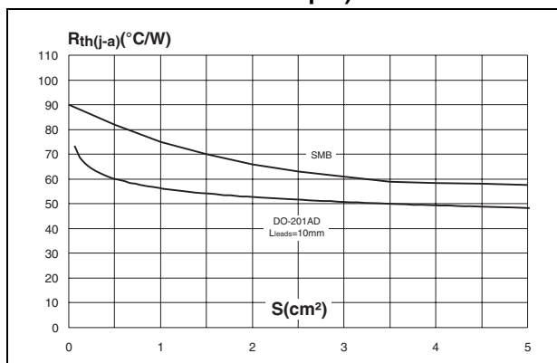
Figure 5. Thermal resistance junction to ambient versus copper surface under each lead (epoxy printed circuit board FR4, copper thickness: 35 \mu\text{m} )
