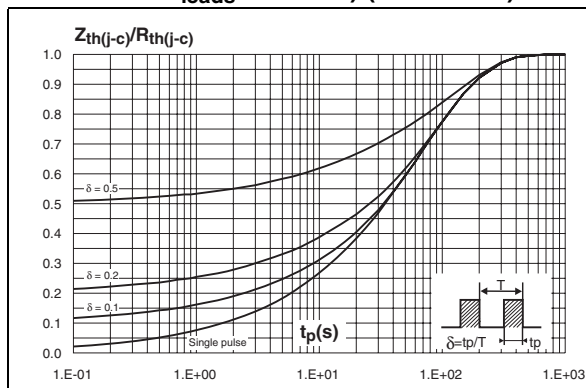
Figure 3. Relative variation of thermal impedance junction ambient versus pulse duration (epoxy FR4, L_{\text{leads}} = 10 \text{ mm} ) (DO-201AD)
