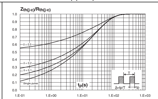
Figure 4. Relative variation of thermal impedance junction ambient versus pulse duration (epoxy FR4, S = 1 \text{ cm}^2 ) (SMC)
