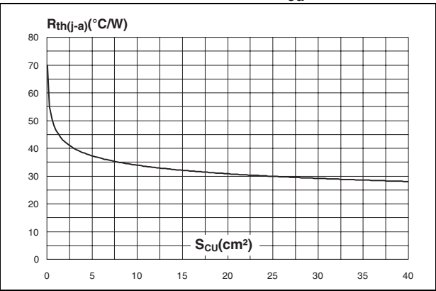
Figure 12. Thermal resistance junction to ambient versus copper surface under each lead (Epoxy printed circuit board FR4, e_{Cu} = 35\text{ }\mu\text{m} )
