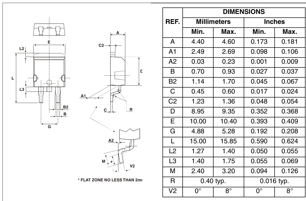
Figure 10: D 2 PAK Package Mechanical Data
