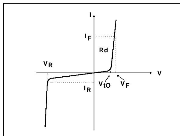
Fig. 6: STATIC CHARACTERISTICS
