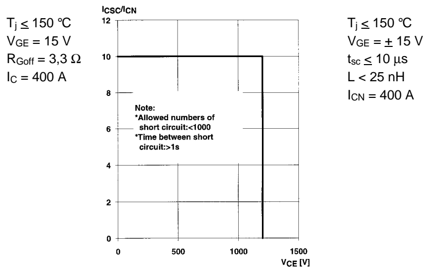
Fig. 6 Safe operating area at short circuit I_C = f(V_{CE})
