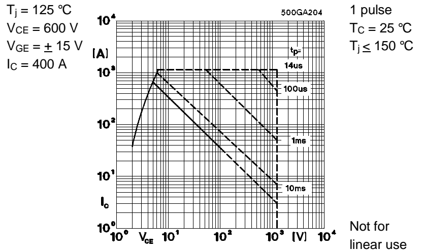
Fig. 4 Maximum safe operating area (SOA) I_C = f(V_{CE})
