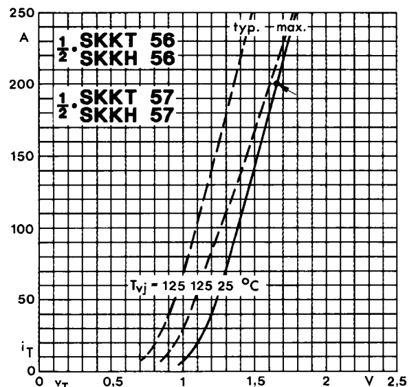
Fig. 8 On-state characteristics
