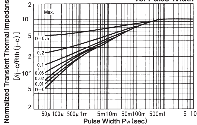
Normalized Transient Thermal Impedance Vs. Pulse Width
