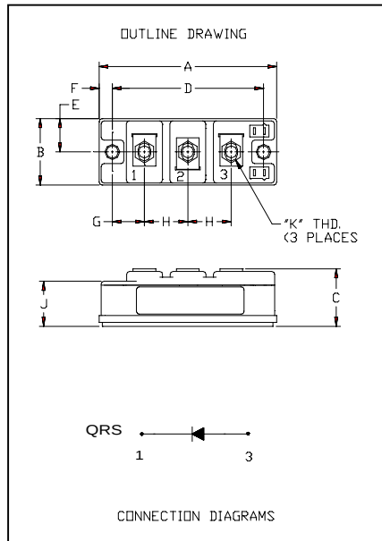
QRS1460T30 Fast Recovery Diode Module 600 Amperes / 1400 Volts
