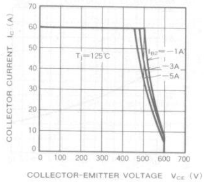
REVERSE BIAS SAFE OPERATING AREA
