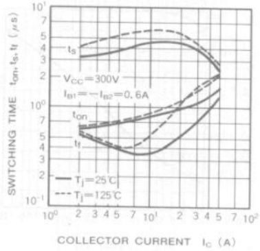
SWITCHING TIME VS. COLLECTOR CURRENT (TYPICAL)
