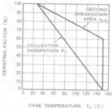
DERATING FACTOR OF F.B.S.O.A.
