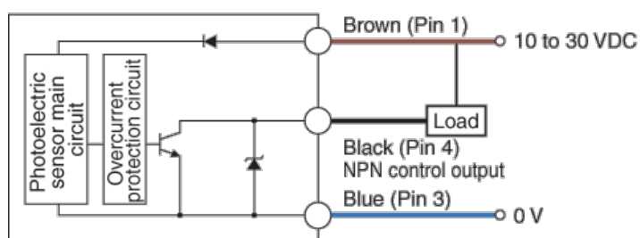
M12 connector PZ-GxxEN
