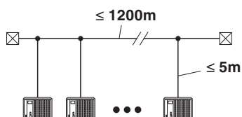
Application drawing
