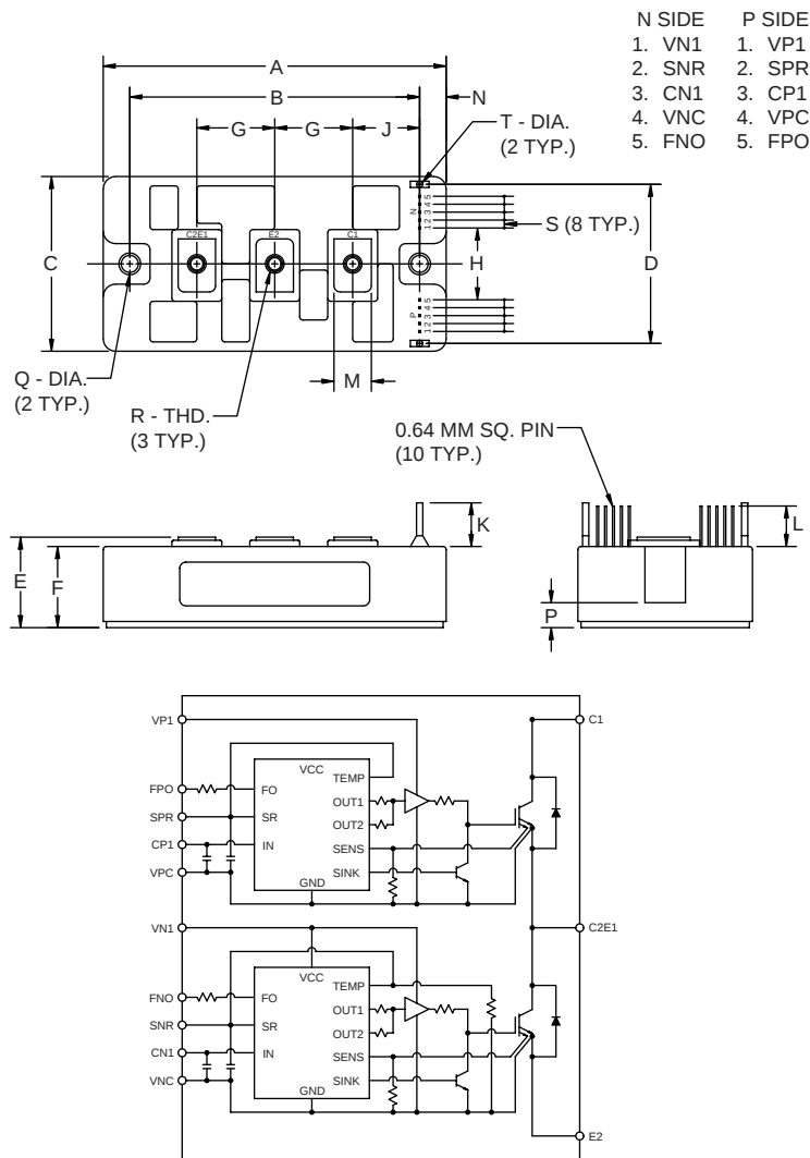
Outline Drawing and Circuit Diagram
