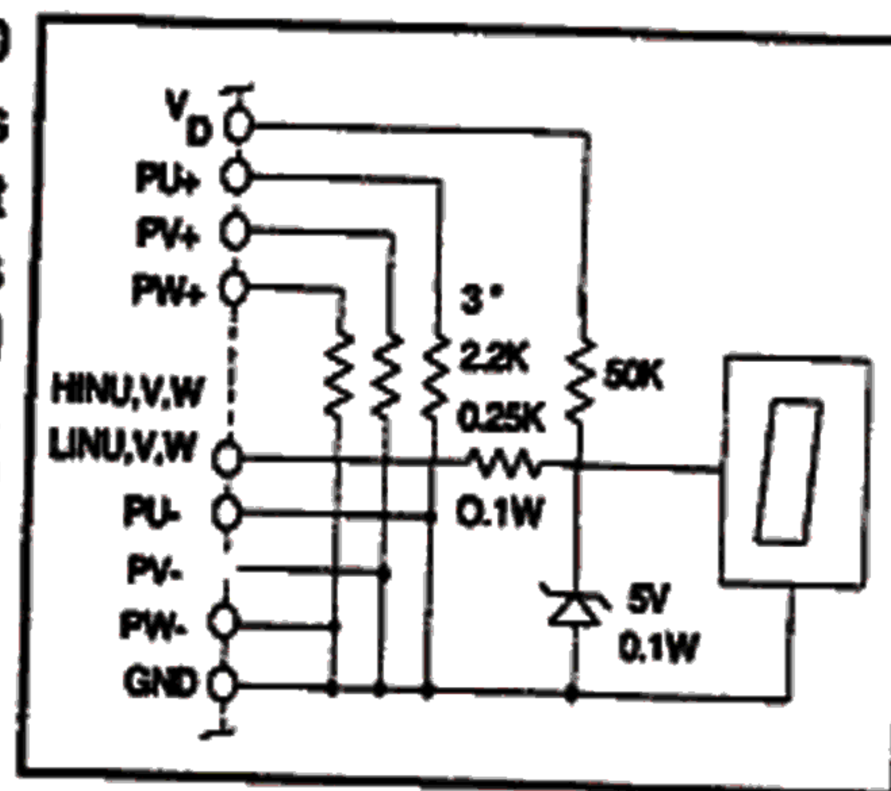
Figure 8 : Input Stage
