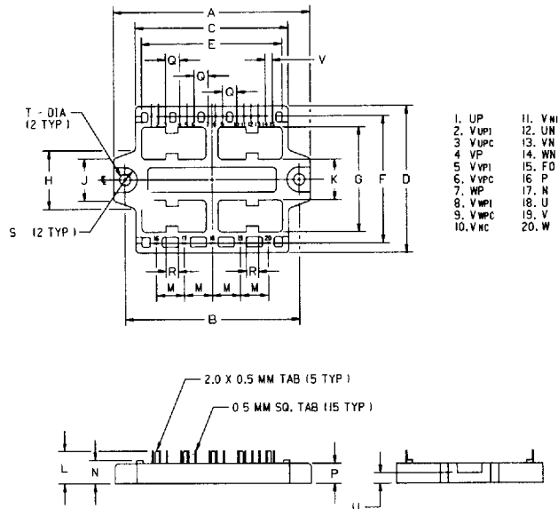
OUTLINE DRAWING
