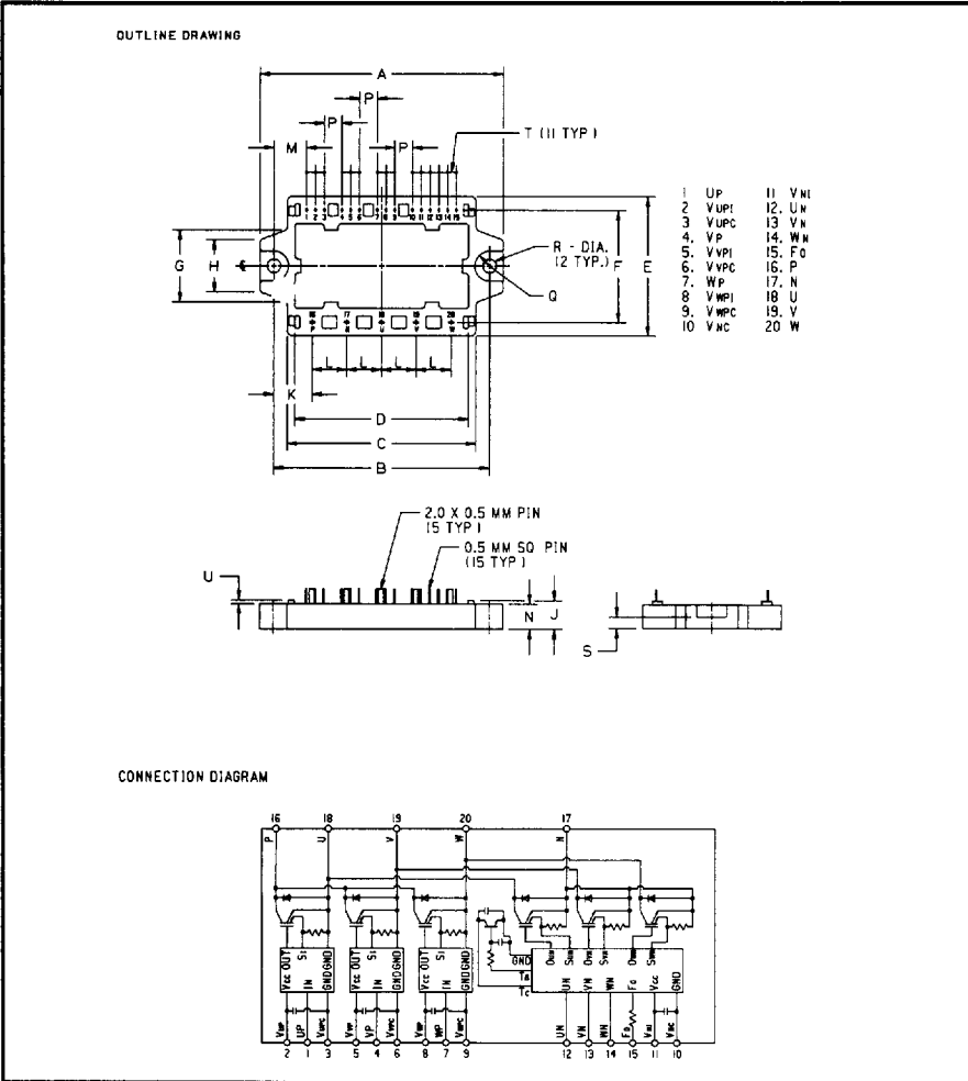
110-230 Volt Line, PM10CHA060 Outline Drawing
