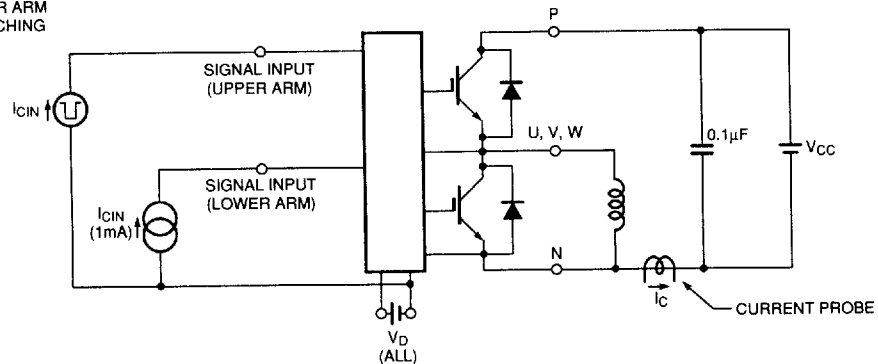
Figure 4 Switching Time Test
