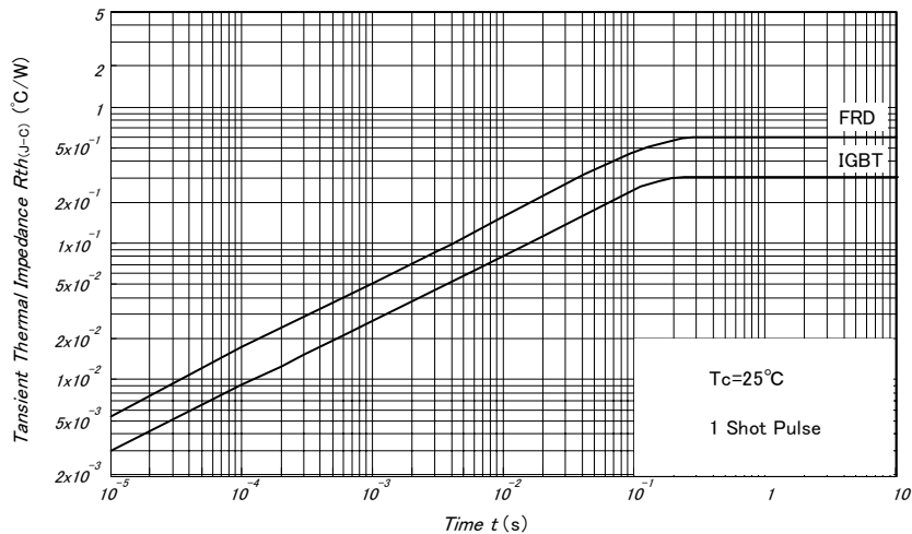
fig11-Transient Thermal Impedance
