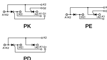
Internal Configurations
