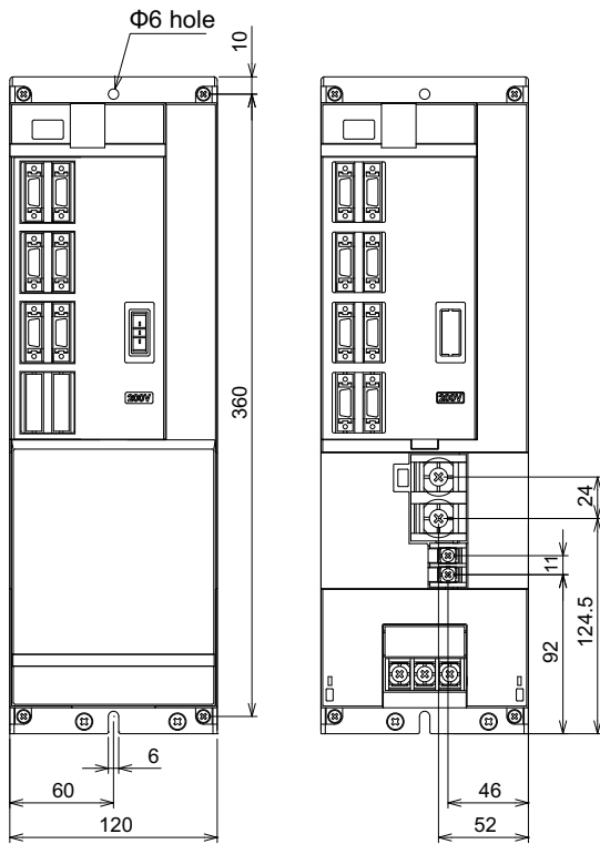
(State with terminal block cover removed)
