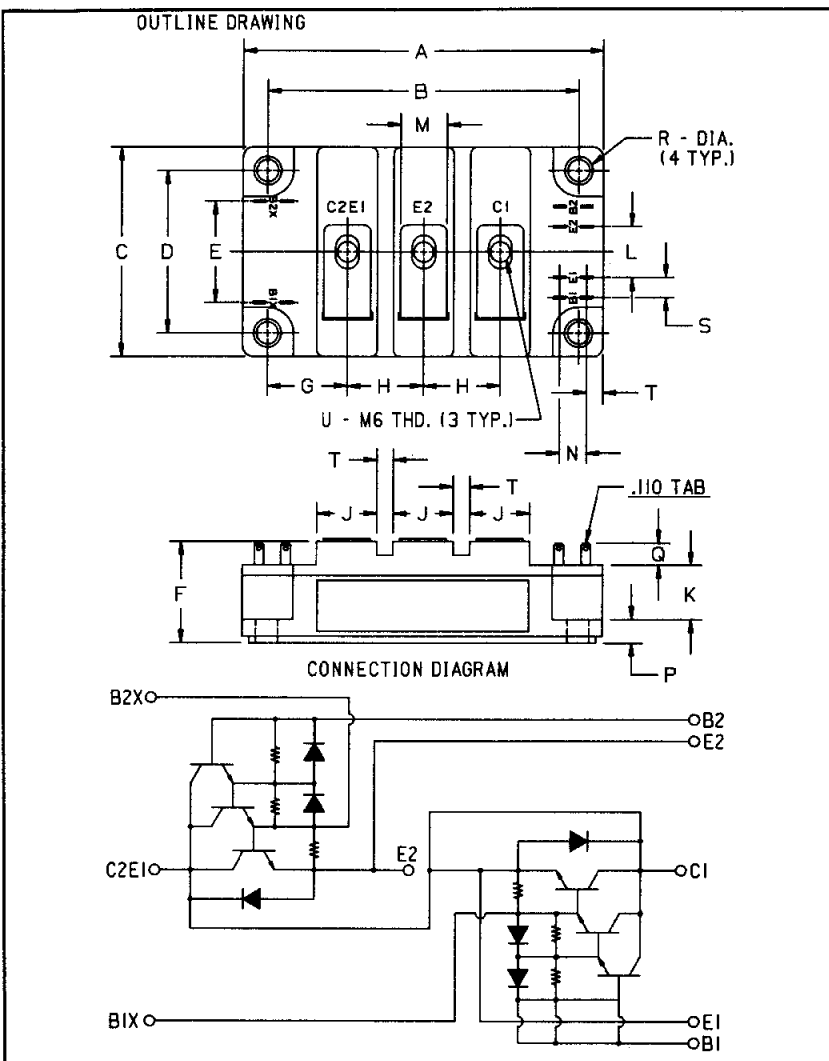
Outline Drawing
