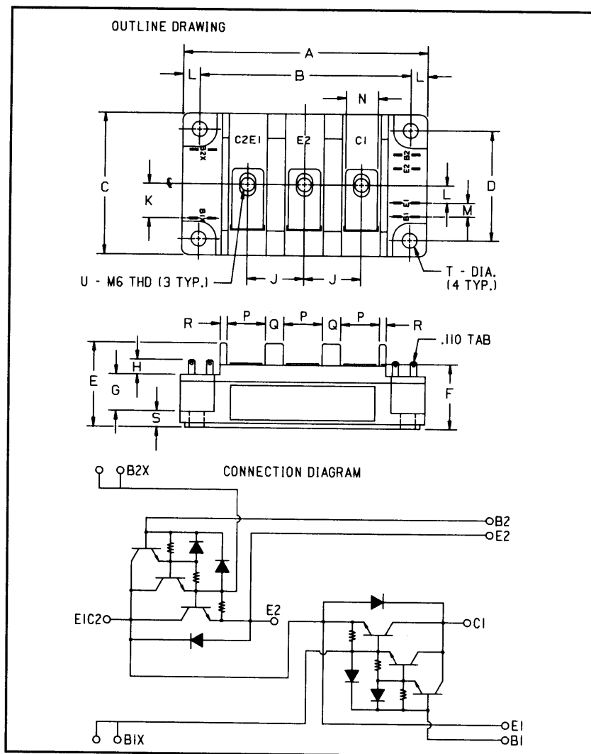
Outline Drawing
