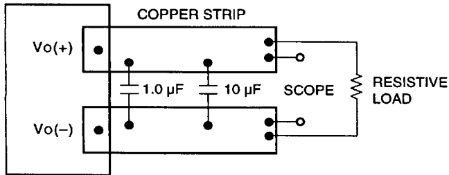
Figure 17. Input Reflected-Ripple Test Setup
