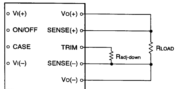
Figure 22. Circuit Configuration to Decrease Output Voltage
