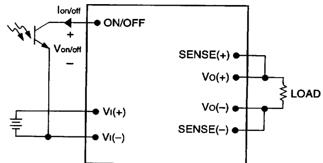
Figure 20. Remote On/Off Implementation B-720 (C).c
