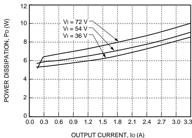
Figure 28. JW050C Power Dissipation vs. Output Current
