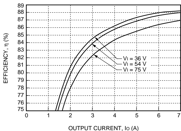
Figure 11. Typical JW100C Converter Efficiency vs. Output Current at Room Temperature
