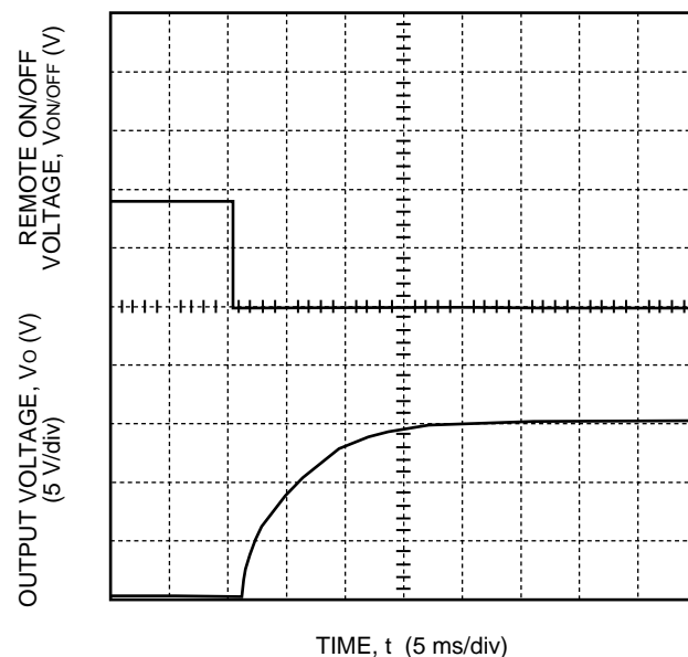
Figure 16. Typical Start-Up from Remote On/Off JW150C1; I_o = I_{o,max}
