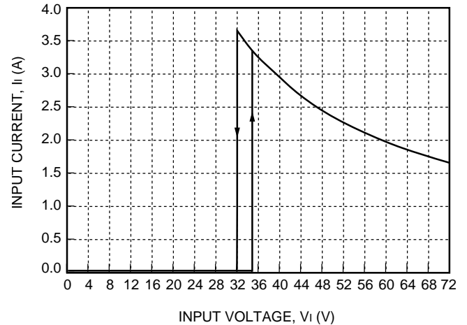
Figure 3. Typical JW100C Input Characteristics at Room Temperature
