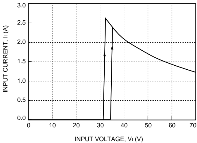
Figure 2. Typical JW075C Input Characteristics at Room Temperature
