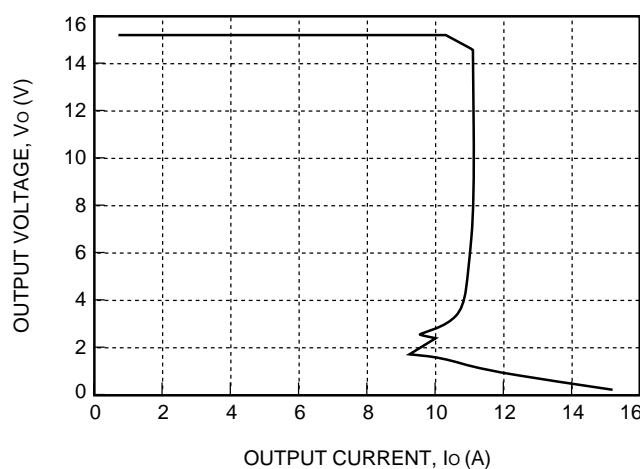
Figure 8. Typical JW150C Output Characteristics at Room Temperature
