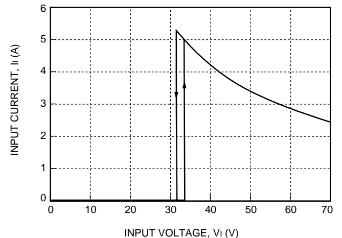
Figure 4. Typical JW150C Input Characteristics at Room Temperature
