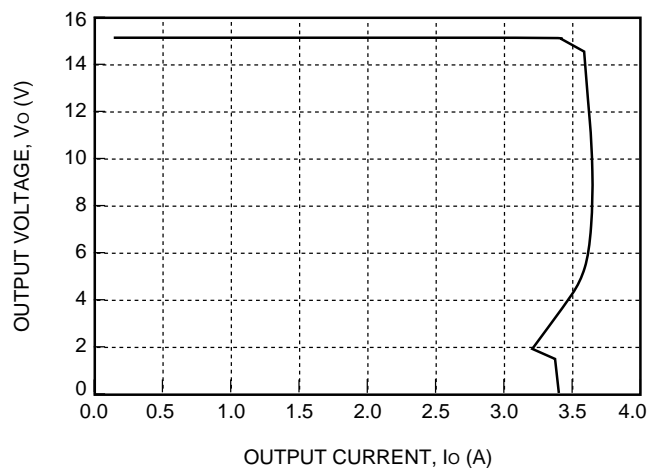
Figure 5. Typical JW050C Output Characteristics at Room Temperature
