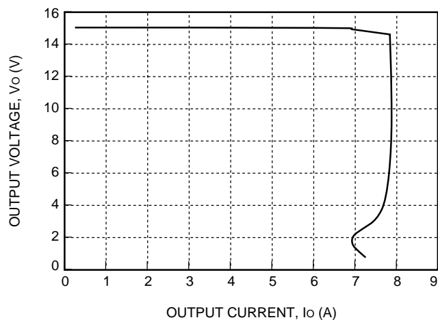
Figure 7. Typical JW100C Output Characteristics at Room Temperature
