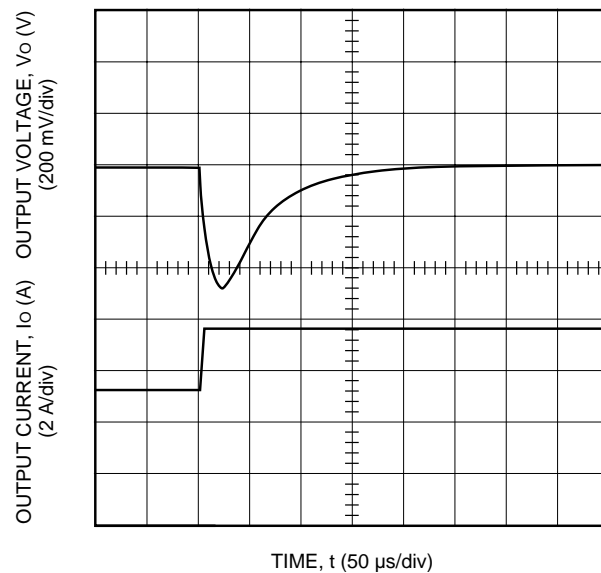
Figure 15. Typical JW150C Transient Response to Step Increase in Load from 50% to 75% of Full Load at Room Temperature and 48 V Input (Waveform Averaged to Eliminate Ripple Component.)
