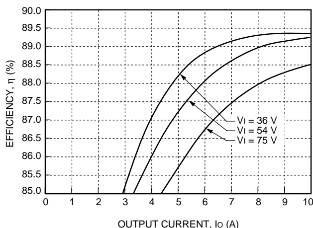
Figure 12. Typical JW150C Converter Efficiency vs. Output Current at Room Temperature
