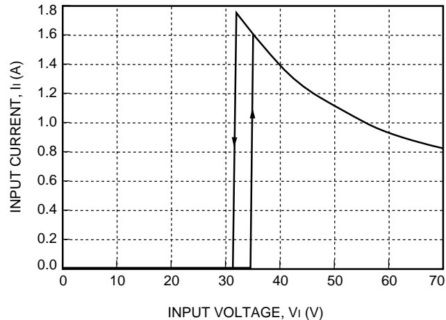
Figure 1. Typical JW050C Input Characteristics at Room Temperature
