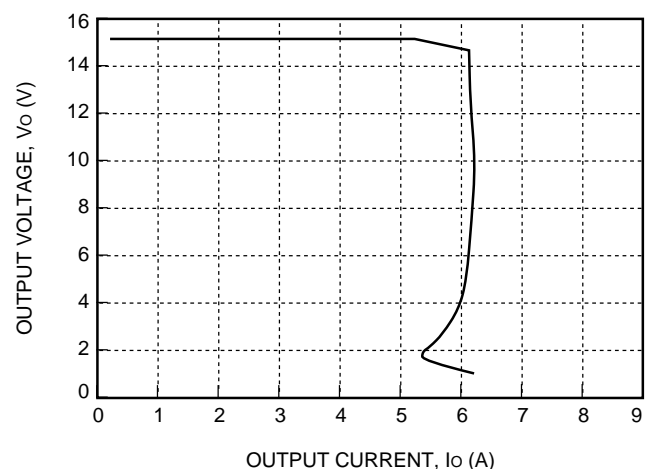
Figure 6. Typical JW075C Output Characteristics at Room Temperature
