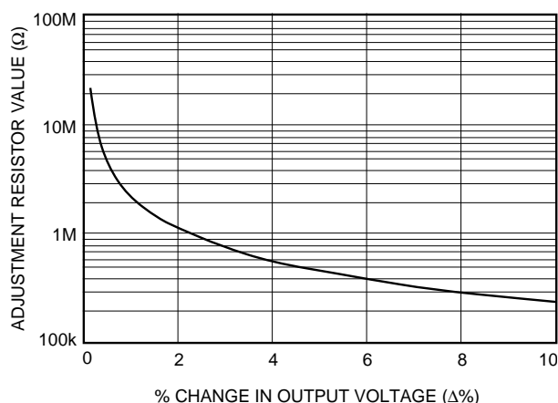
Figure 23. Resistor Selection for Increased Output Voltage
