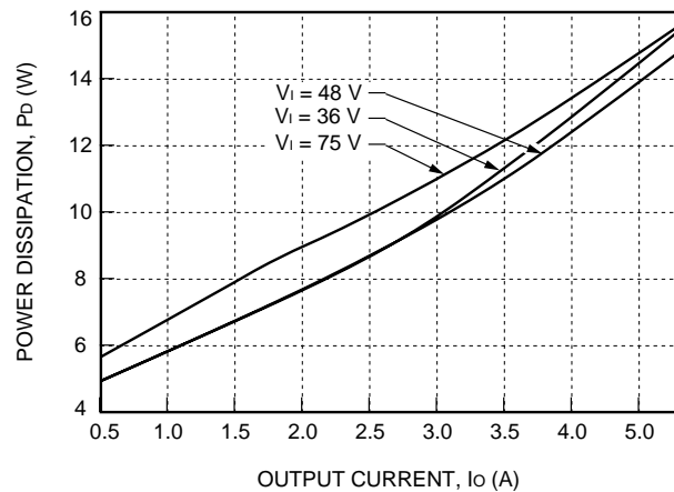
Figure 27. JW150R Power Dissipation vs. Output Current
