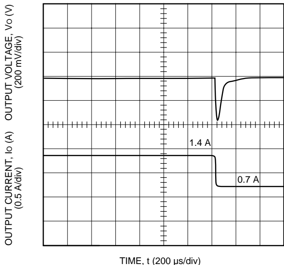
Figure 9. Typical JW075R Transient Response to Step Decrease in Load from 50% to 25% of Full Load at Room Temperature and 48 Vdc Input (Waveform Averaged to Eliminate Ripple Component.)
