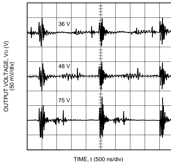
Figure 7. Typical JW075R Output Ripple Voltage at Room Temperature, 36 Vdc to 75 V Input, and 30 A Output
