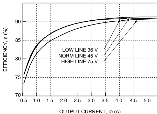
Figure 6. Typical JW150R Converter Efficiency vs. Output Current at Room Temperature
