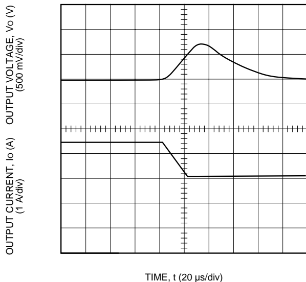
Figure 10. Typical JW150R Transient Response to Step Decrease in Load from 50% to 25% of Full Load at Room Temperature and 48 Vdc Input (Waveform Averaged to Eliminate Ripple Component.)
