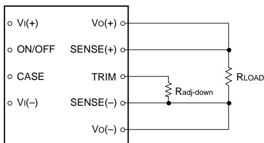
Figure 20. Circuit Configuration to Decrease Output Voltage
