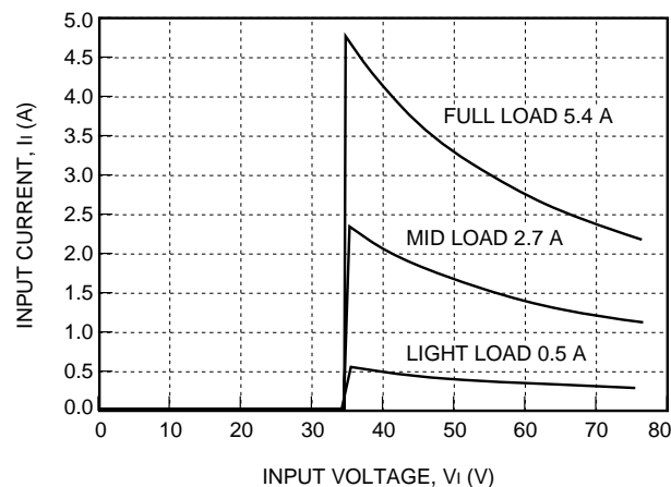
Figure 2. Typical JW150R Input Characteristics at Room Temperature
