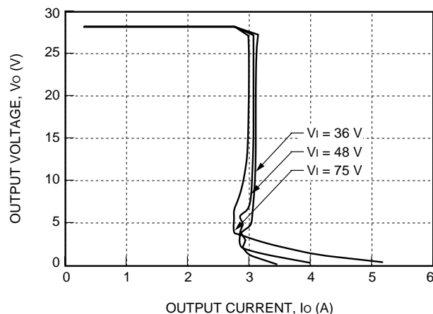
Figure 3. Typical JW075R Output Characteristics at Room Temperature
