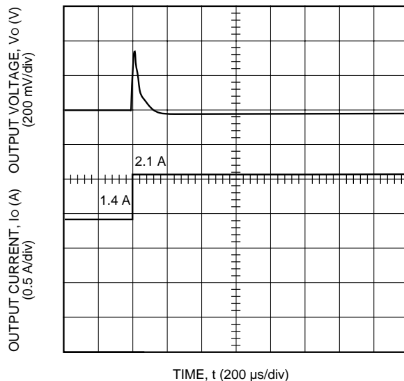
Figure 11. Typical JW075R Transient Response to Step Increase in Load from 50% to 75% of Full Load at Room Temperature and 48 Vdc Input (Waveform Averaged to Eliminate Ripple Component.)
