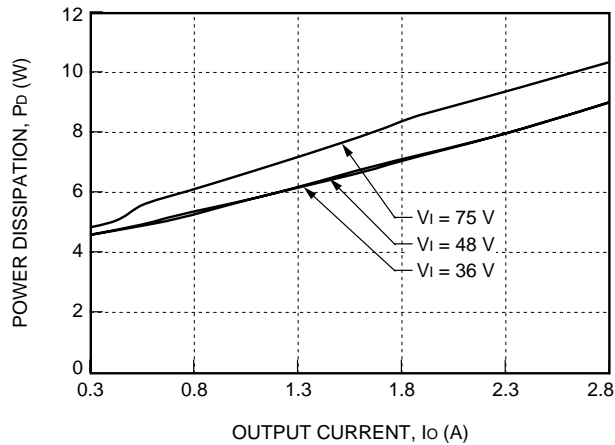
Figure 26. JW075R Power Dissipation vs. Output Current
