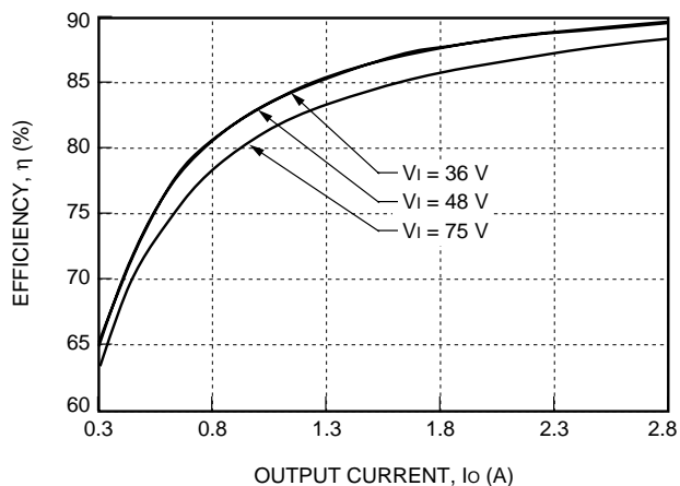
Figure 5. Typical JW075R Converter Efficiency vs. Output Current at Room Temperature
