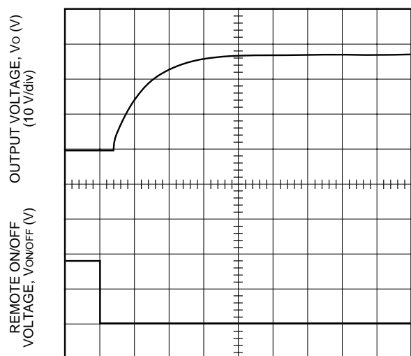
Figure 13. Typical Start-Up from Remote On/Off JW075R1; I_o = Full Load
