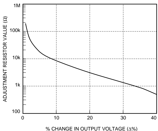
Figure 21. Resistor Selection for Decreased Output Voltage
