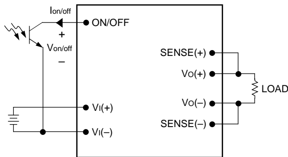
Figure 19. Effective Circuit Configuration for Single-Module Remote-Sense Operation
