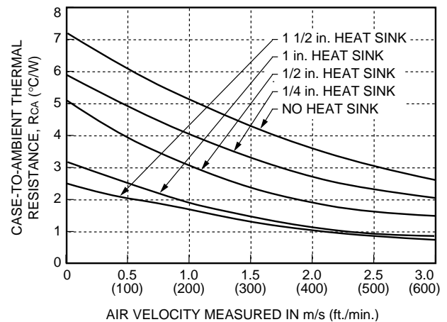
Figure 28. Case-to-Ambient Thermal Resistance Curves; Either Orientation
