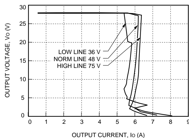
Figure 4. Typical JW150R Output Characteristics at Room Temperature
