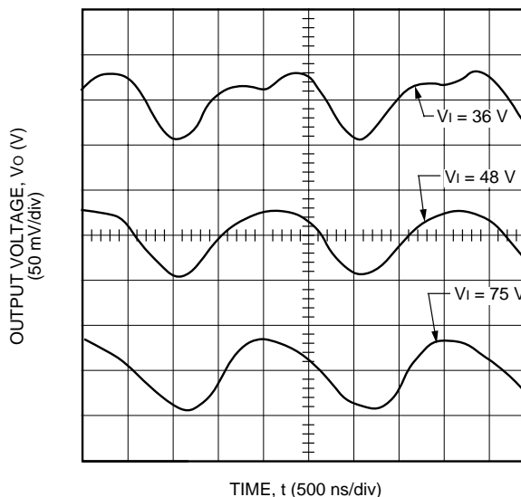
Figure 8. Typical JW150R Output Ripple Voltage at Room Temperature, 36 Vdc to 75 V Input, and 5.4 A Output
