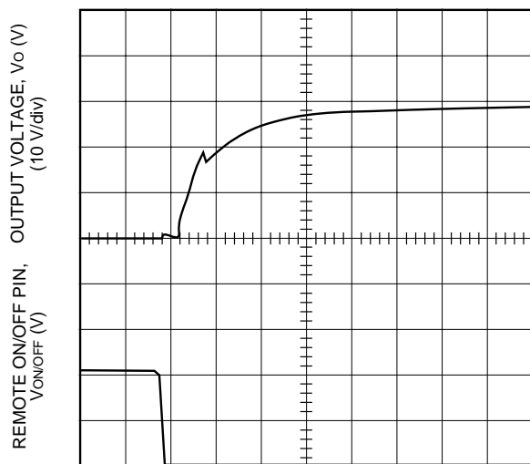
Figure 14. Typical Start-Up from Remote On/Off JW150R; I_o = Full Load
