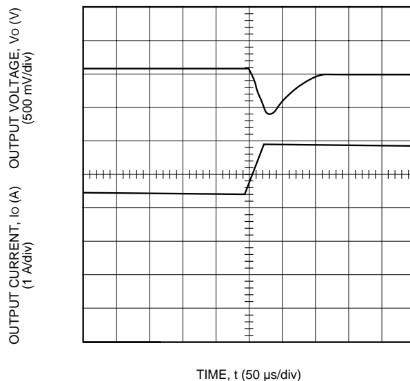
Figure 12. Typical JW150R Transient Response to Step Increase in Load from 50% to 75% of Full Load at Room Temperature and 48 Vdc Input (Waveform Averaged to Eliminate Ripple Component.)
