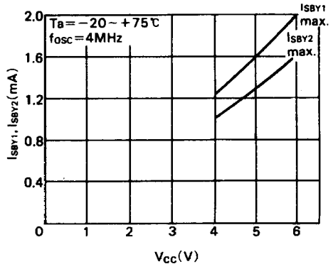
I_{SBY} vs. V_{CC} Characteristics (Resistor Oscillator Option)
