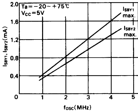
I_{SBY} vs. f_{osc} Characteristics (Resistor Oscillator Option)
