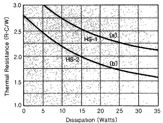
Figure 2. Thermal Resistance Models HS-1 & HS-2
