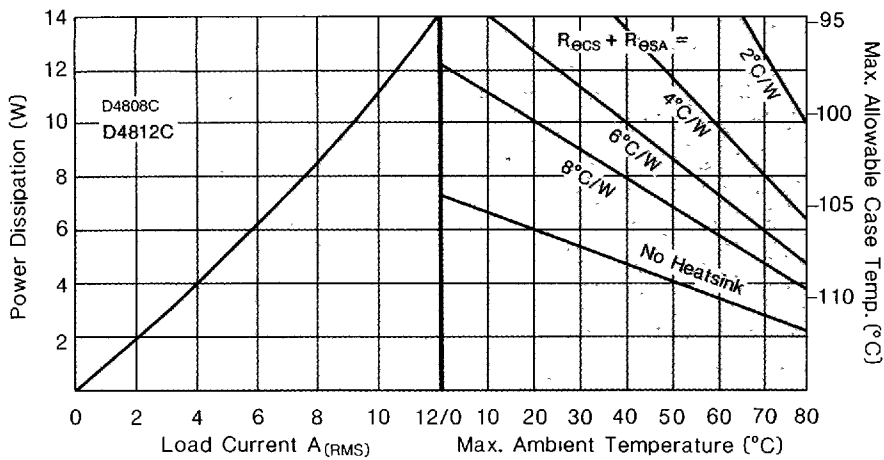
Figure 4. Thermal Derating Curves: 8 & 12 Amp., 480V
