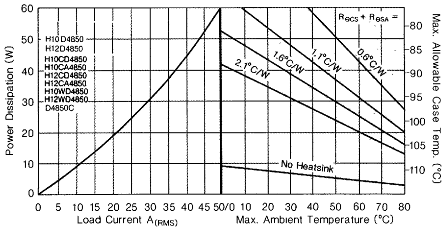
Figure 6. Thermal Derating Curves: 50 Amp., 480V
