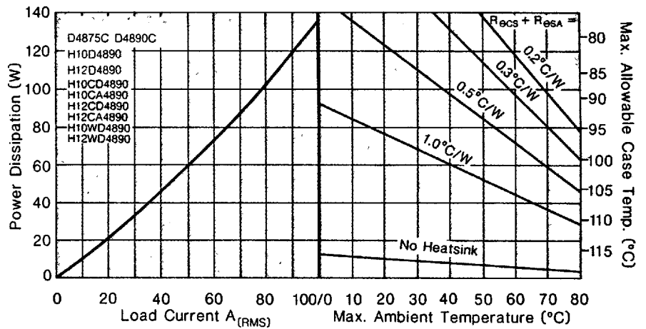
Figure 11. Thermal Derating Curves: 75 & 90 Amp., 480V
