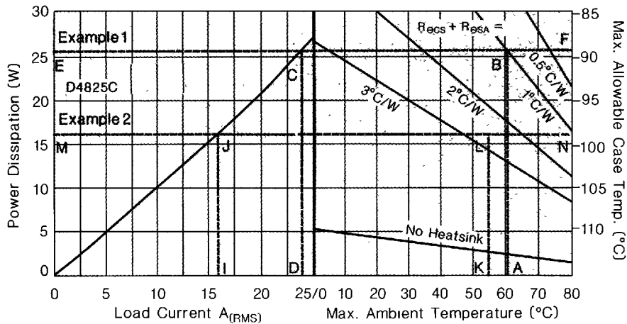
Figure 5. Thermal Derating Curves: 25 Amp., 480V
