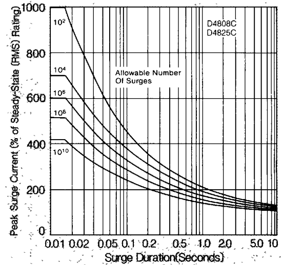
Figure 7. Peak Surge Current vs. Duration: 8 and 25 Amp Models.
