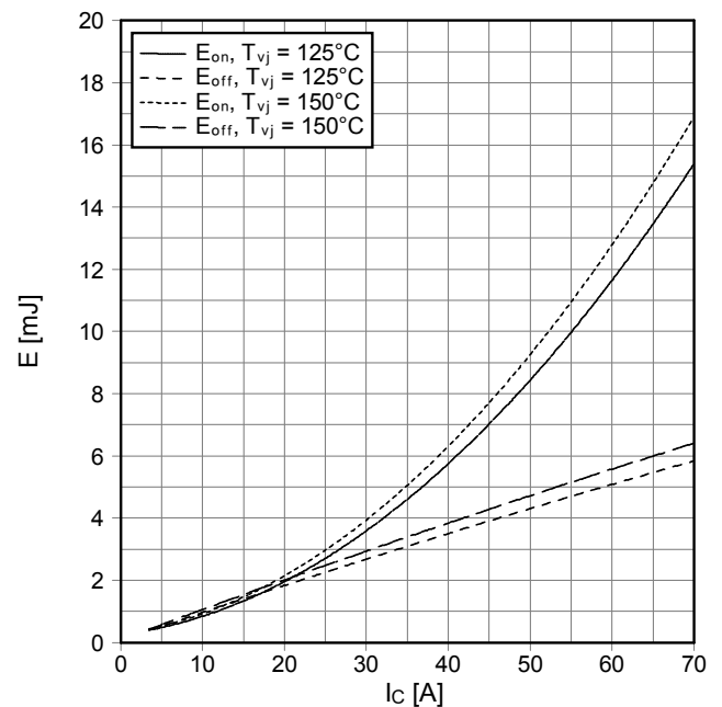
Schaltverluste IGBT-Wechselr. (typisch) switching losses IGBT-inverter (typical) E_{on} = f(I_c), E_{off} = f(I_c) V_{GE} = \pm 15\text{ V}, R_{Gon} = 13\ \Omega, R_{Goff} = 13\ \Omega, V_{CE} = 600\text{ V}
