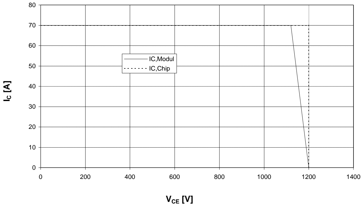
Sicherer Arbeitsbereich Wechsell. (RBSOA) I_C = f(V_{CE}) Reverse bias safe operating area Inverter (RBSOA) T_{vi} = 125^\circ\text{C} , V_{GE} = \pm 15\text{V} , R_G = 22\ \Omega
