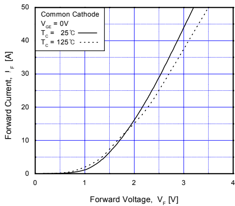
Fig 17. Forward Characteristics
