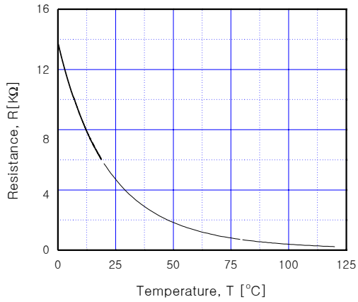
Fig 21. NTC Characteristics
