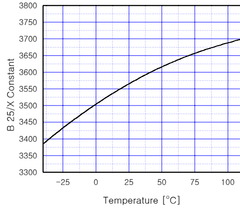
Fig 22. NTC Characteristics
