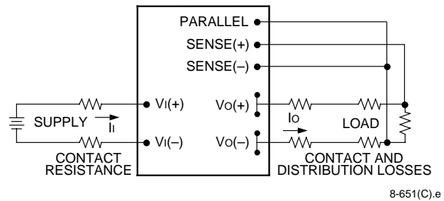
Figure 11. Effective Circuit Configuration for Single-Module Remote-Sense Operation
