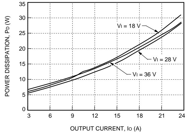
Figure 20. Power Dissipation as Heat vs. Output Current
