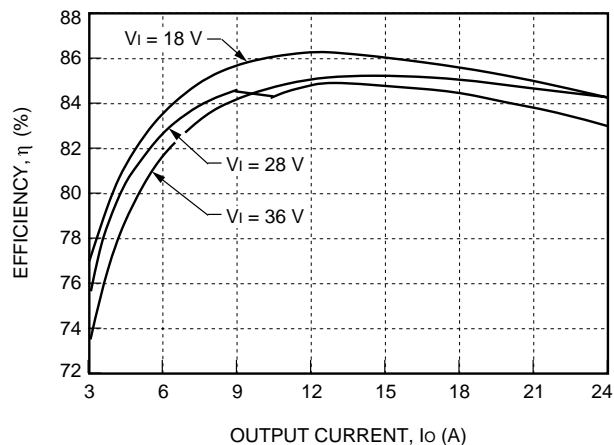
Figure 3. Typical FC150S6R5 Efficiency vs. Output Current at Room Temperature
