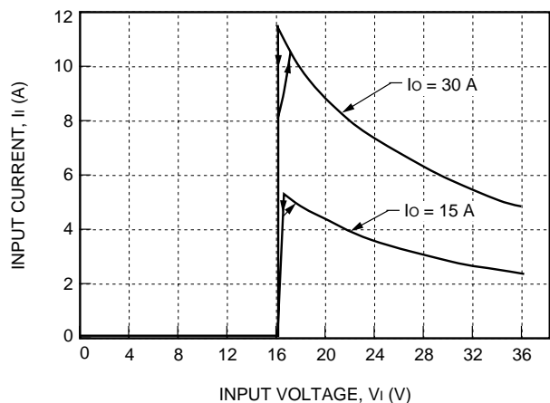
Figure 1. Typical FC150S6R5 Input Characteristics at Room Temperature
