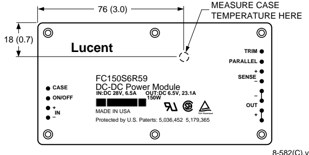
Figure 16. Case Temperature Measurement Location
