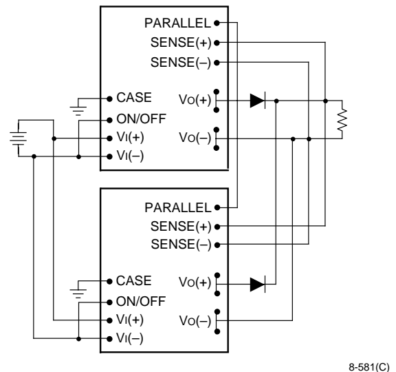
Figure 15. Wiring Configuration for Redundant Parallel Operation
