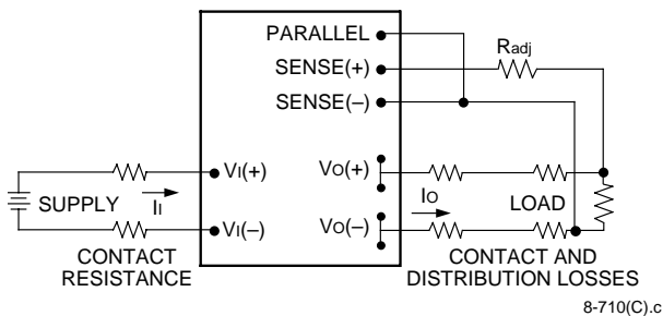
Figure 14. Circuit Configuration to Adjust Output Voltage
