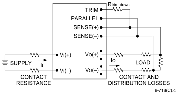
Figure 13. Circuit Configuration to Trim Down Output Voltage
