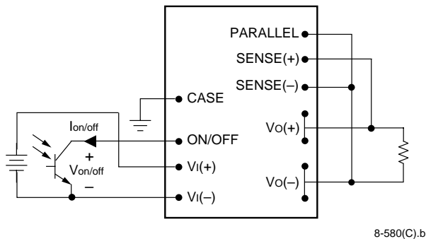
Figure 10. Remote On/Off Implementation
