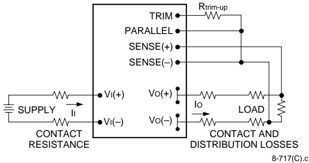
Figure 12. Circuit Configuration to Trim Up Output Voltage
