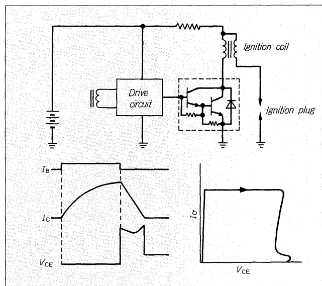
Fig. 1 Fundamental circuit of the ignition system and its functioning
