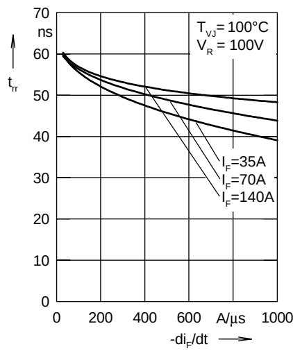
Fig. 5 Typ. recovery time t_{tr} versus -di_F/dt
