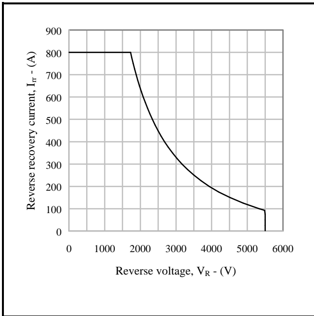
Fig.7 RBSOA
