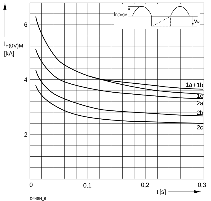
Bild / Fig. 4 Grenzstrom / Maximum overload forward current I_{F(0V)M} = f(t) 1 - I_{FAV(vor)} = 0\text{ A} ; t_{vj} = t_c = 25\text{ °C} 2 - I_{FAV(vor)} = 450\text{ A} ; t_c = 122\text{ °C} ; t_{vj} = 180\text{ °C} a - V_R \leq 50\text{ V} b - V_R = 0,5 V_{RRM} c - V_R = 0,8 V_{RRM}
