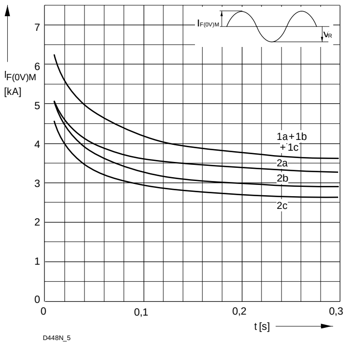
Bild / Fig. 3 Grenzstrom / Maximum overload forward current I_{F(0V)M} = f(t) 1 - I_{FAV(vor)} = 0\text{ A} ; t_{vj} = t_c = 25\text{ °C} 2 - I_{FAV(vor)} = 450\text{ A} ; t_c = 122\text{ °C} ; t_{vj} = 180\text{ °C} a - V_R \leq 50\text{ V} b - V_R = 0,5 V_{RRM} c - V_R = 0,8 V_{RRM}
