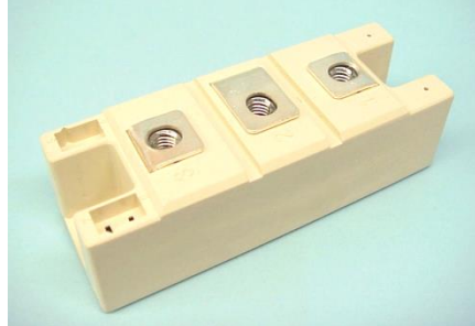
CD61__16B, CS61__16B CN61__16B, CC61__16B Dual & Single Diode Isolated POW-R-BLOK™ Module 160 Amperes / Up to 2200 Volts
