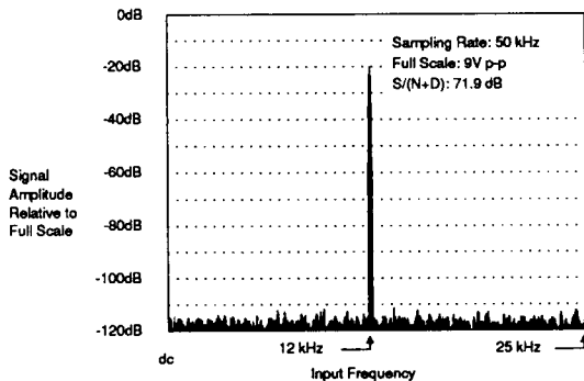
Figure 34. CS5016 FFT plot with 12 kHz -20 dB Input
