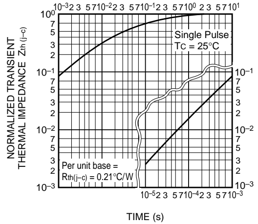
TRANSIENT THERMAL IMPEDANCE CHARACTERISTICS (IGBT part)
