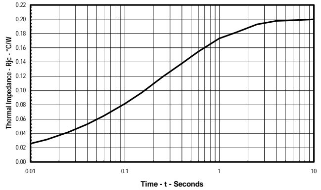
Maximum Transient Thermal Impedance (Junction to Case, Per Diode)
