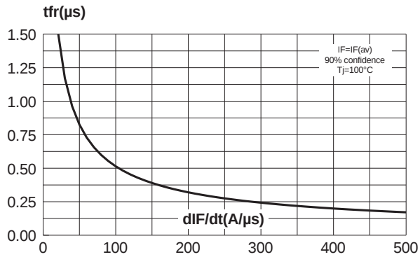
Fig. 11: Forward recovery time versus dl_F/dt (per diode)
