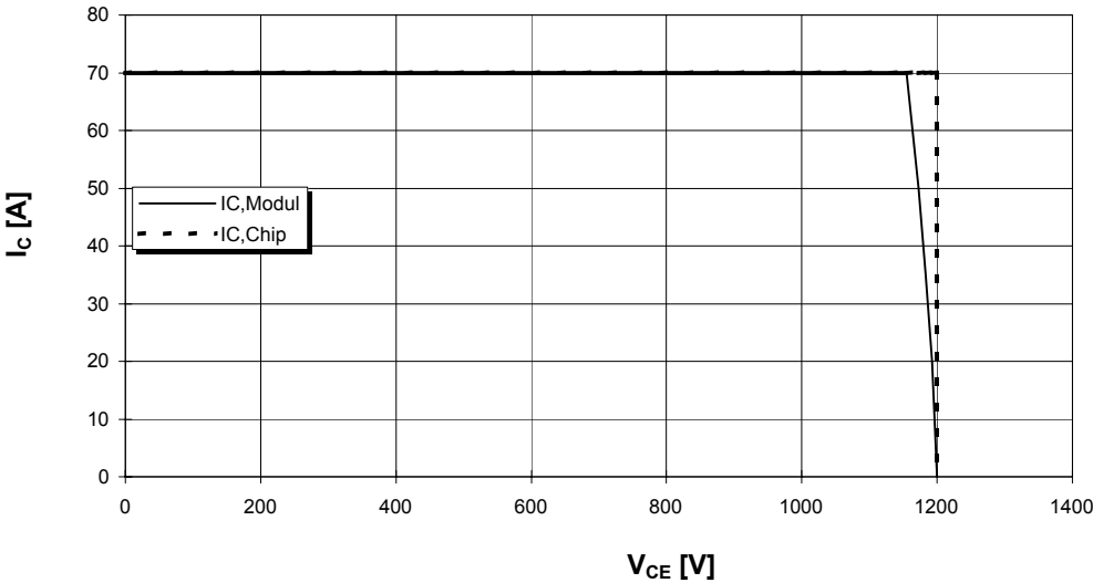
Sicherer Arbeitsbereich (RBSOA) Reverse bias safe operation area (RBSOA) V_{GE} = 15V, R_G = 22 \Omega, T_{vj} = 125^\circ C
