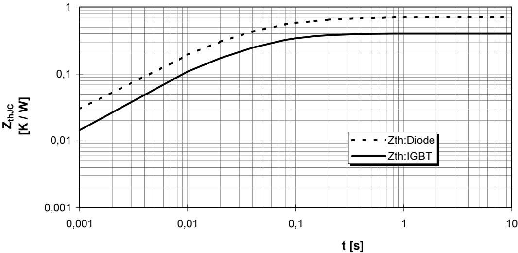
Transienter Wärmewiderstand Z_{thJC} = f(t) Transient thermal impedance
