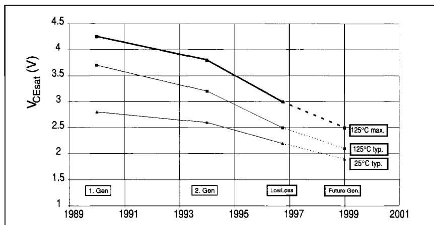
Figure 1. On-State Voltage Trend of 1200V IGBTs.
