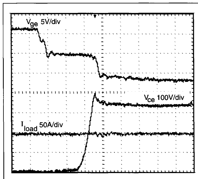
Figure 2(b). Turn-Off With Inductive Load, T_c=25^{\circ}\text{C} .
