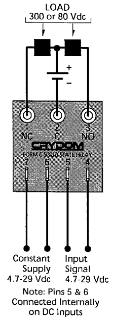
DC300S6-C, DC80S15-C, DC300S15-C, DC INPUT & OUTPUT
