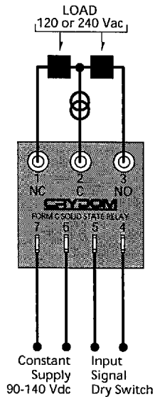
A2415-C, A2440-C DRY SWITCH CONTROL, AC OUTPUT
