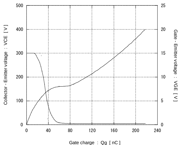
[ Inverter ] Dynamic Gate charge (typ.) V_{CC} = 300\text{V} , I_C = 30\text{A} , T_j = 25^\circ\text{C}
