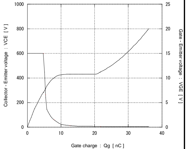
[ Inverter ] Dynamic Gate charge (typ.) Vcc=600V, Ic=10A, T j = 25°C
