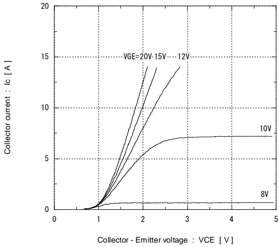
[ Inverter ] Collector current vs. Collector-Emitter voltage T j = 25°C (typ.) / chip
