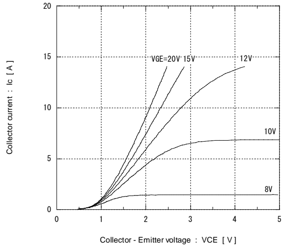
[ Inverter ] Collector current vs. Collector-Emitter voltage T j = 125°C (typ.) / chip
