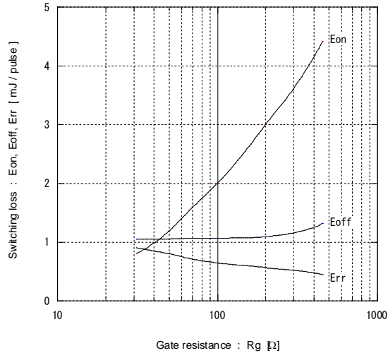
[ Inverter ] Switching loss vs. Gate resistance (typ.) Vcc=600V, Ic=10A, VGE=+15V, Tj= 125°C
