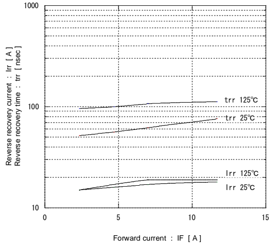
[ Inverter ] Reverse recovery characteristics (typ.) Vcc=600V, VGE=+15V, Rg=100Ω
