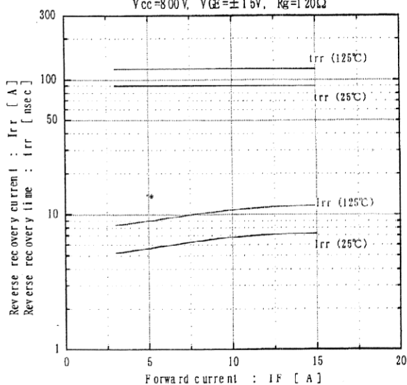
[ Inverter ] Reverse recovery characteristics (typ.) V_{CC}=800V , V_{GE}=\pm 15V , R_g=120\Omega
