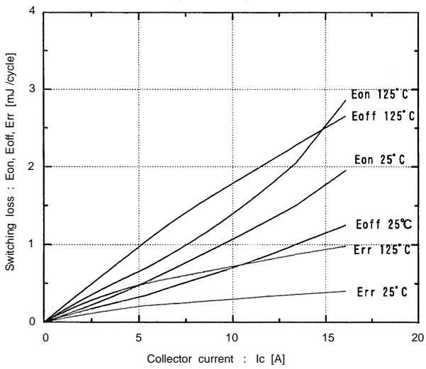
Switching loss vs. Collector current V_{cc}=600V , R_G=62\ \Omega , V_{GE}=\pm 15V
